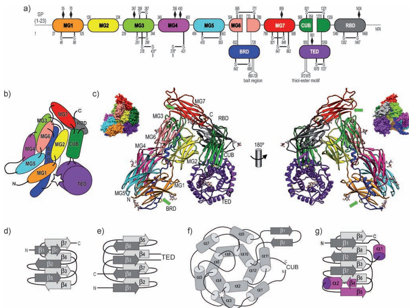
Figure 1. a) Domain organization of human \alpha_2 M depicting the flanking residues of each domain, the disulfide bonds, the N-linked glycosylation sites (as black rhombuses), and the insertion sites of the bait region and the thioester. b) Approximate arrangement of the domains constituting the \alpha_2 M-MA monomer in front view. The thioester site is shown as a white star. The flexible bait region is depicted as a dashed line. c) Connolly surface and Richardson-type plot of an \alpha_2 M-MA monomer in front view (convex face; left) and in back view (concave face; right). Green arrows pinpoint the anchor points of the flexible bait region. d–g) Topology scheme with secondary-structure element nomenclature of the MG domains (d), the CUB domain (e), the TED domain (f), and the RBD domain (g). The elements distinguishing RBD from MGs are shown in magenta.
